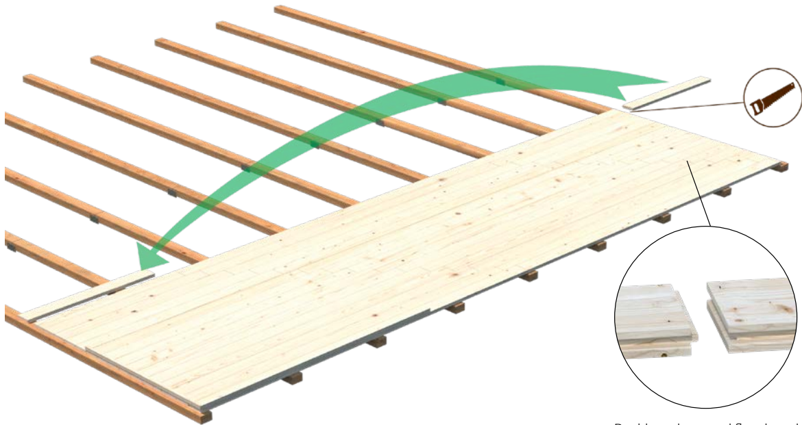
Double end tenoned floor board
