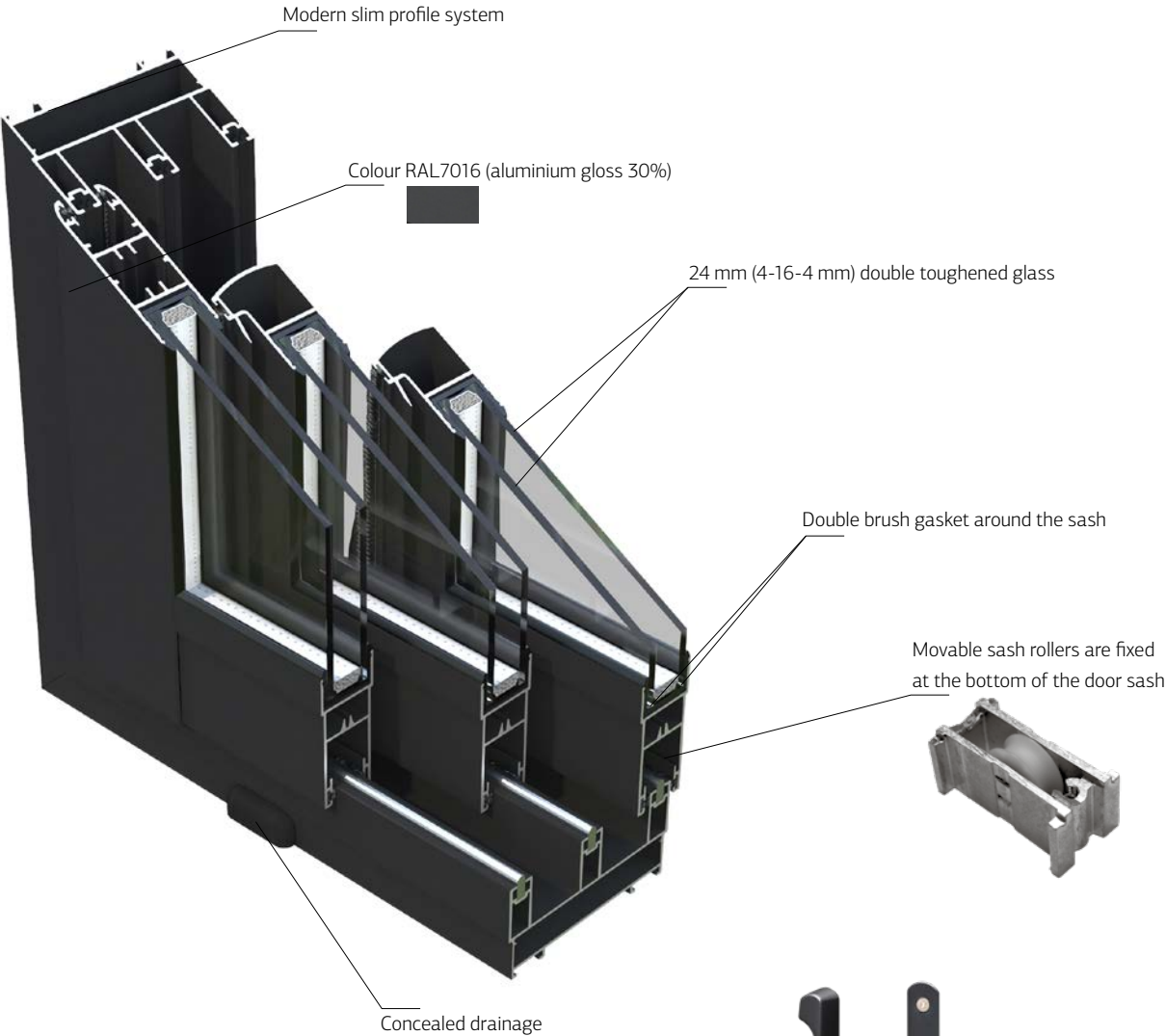
A sliding door system with two or three leafs
