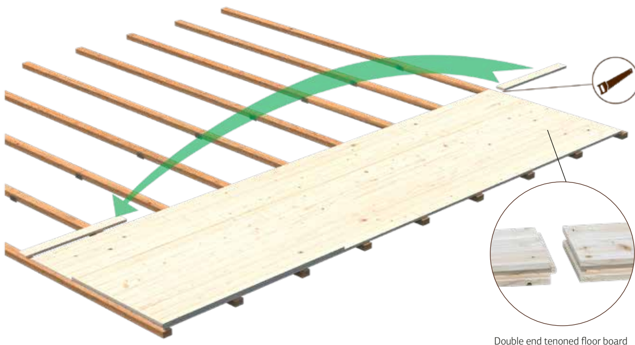
Double end tenoned floor board
